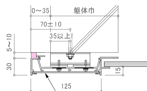
SM125R(RC用)
